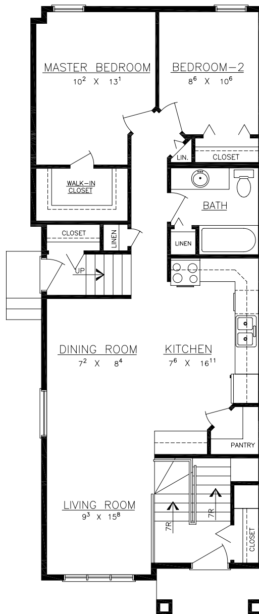
FLOOR PLAN
